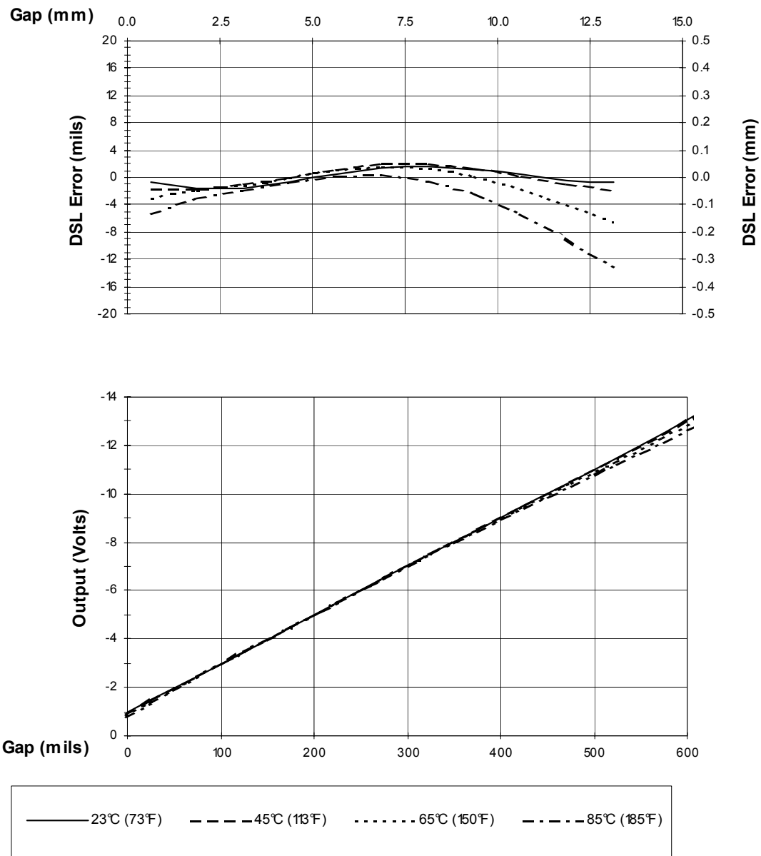
Figure 6 Typical 3300 XL 25 mm 5 m Proximator® Sensor with 4 m Extension Cable @ High Temperature (Probe is at 25°C)
