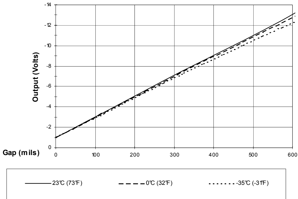
Figure 7 Typical 3300 XL 25 mm 9 m Proximity® Sensor with 8 m of Extension Cable @ Low Temperature (Probe is at 25°C)
